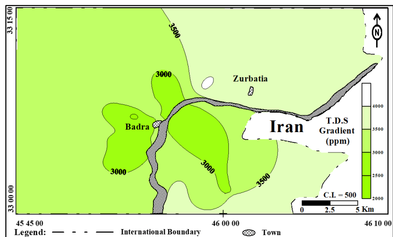
Figure 7 Groundwater salinity distribution map of unconfined aquifer
