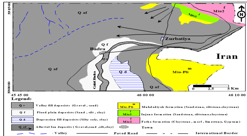
Figure 2 Geological map of the area modified after [10]
