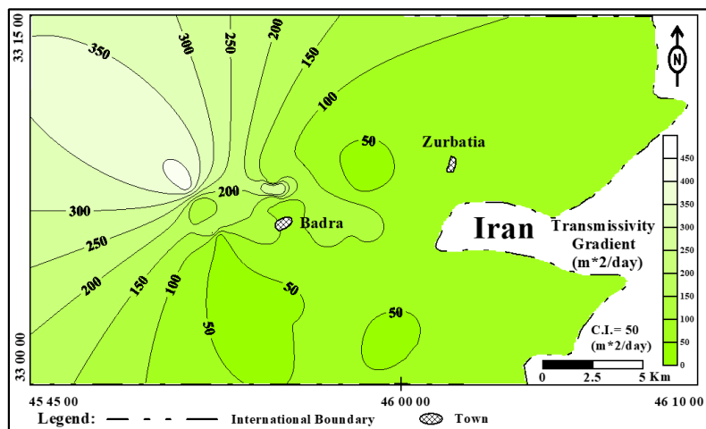
Figure 4 Transmissivity map of the unconfined aquifer
