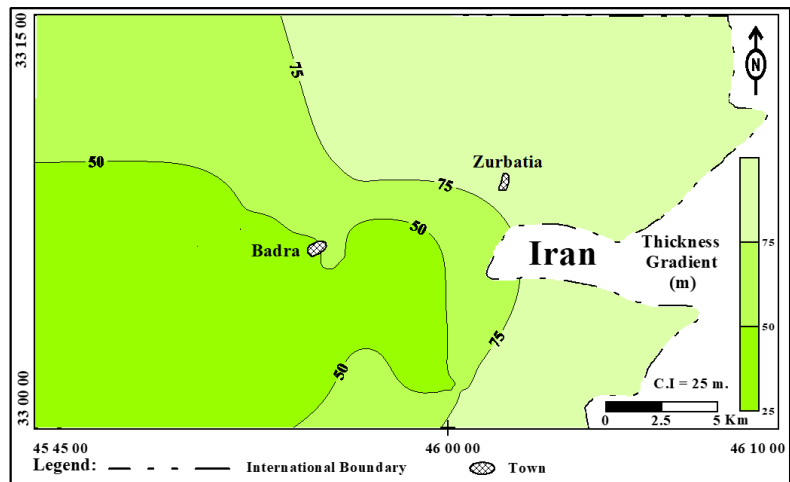
Figure 3 Thickness map of the unconfined aquifer
