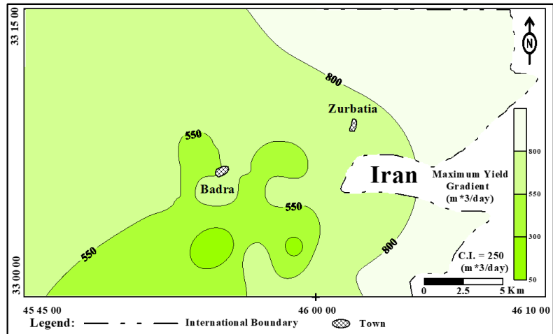
Figure 5 Maximum yields map of the unconfined aquifer
