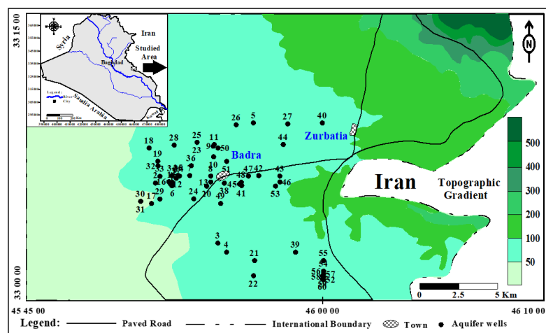
Figure 1 Location and topographic map of studied area
