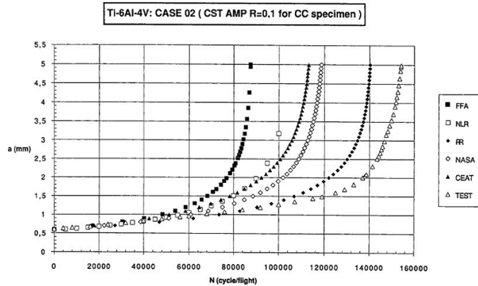
Figure 8 Ti-6Al-4V case 02
